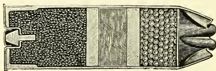
Brass Cartridge Case Wadded for Close Shooting.
